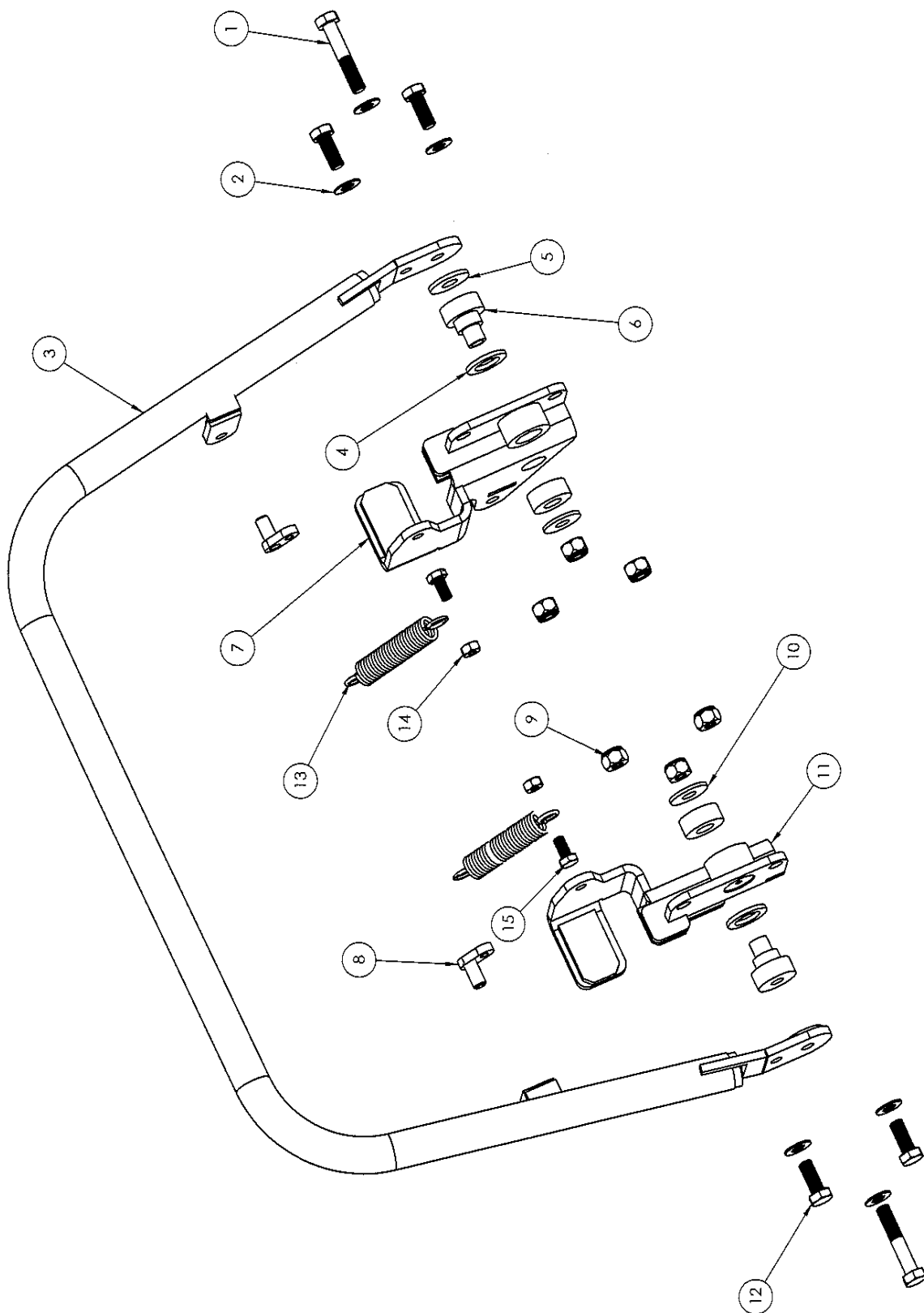
Fig 7: Bottom Handle Assembly
