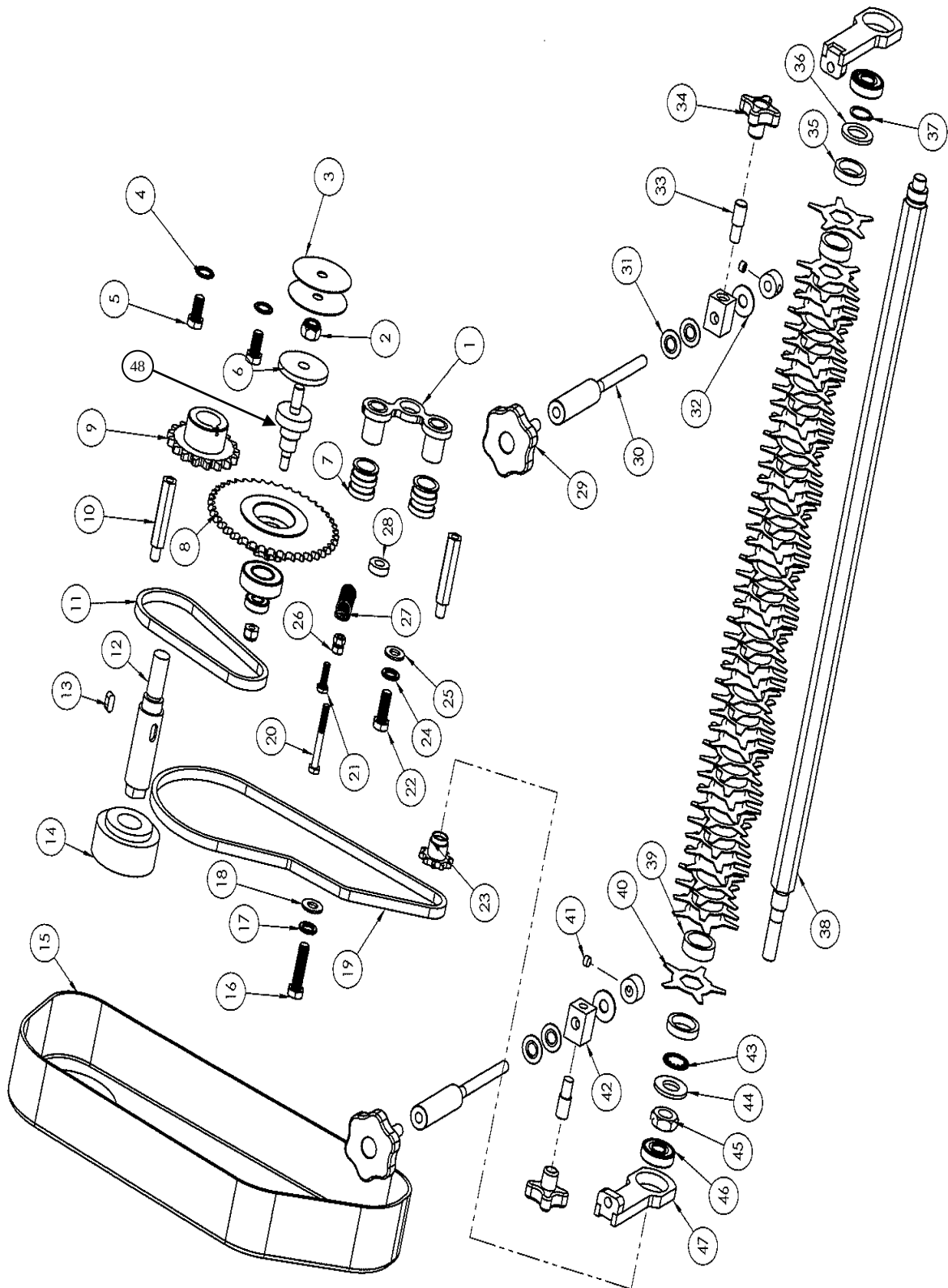
Fig 9: Groomer/Rotary Brush Drive Assembly (Tournament 20" & 24" Only)
