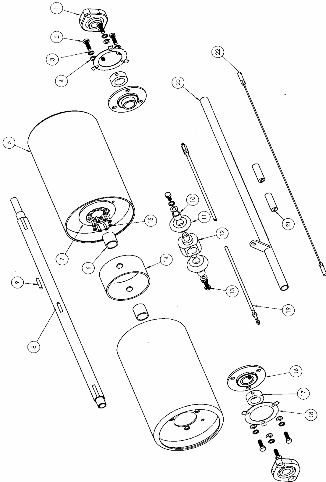
Fig 4: Rear Roller Assembly
