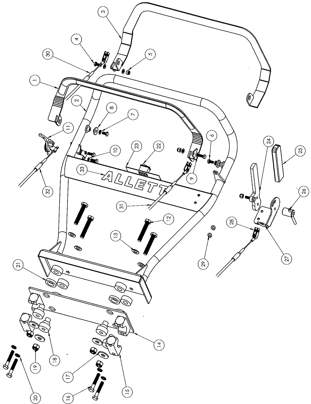
Fig 6: Top Handle Bar Assembly
