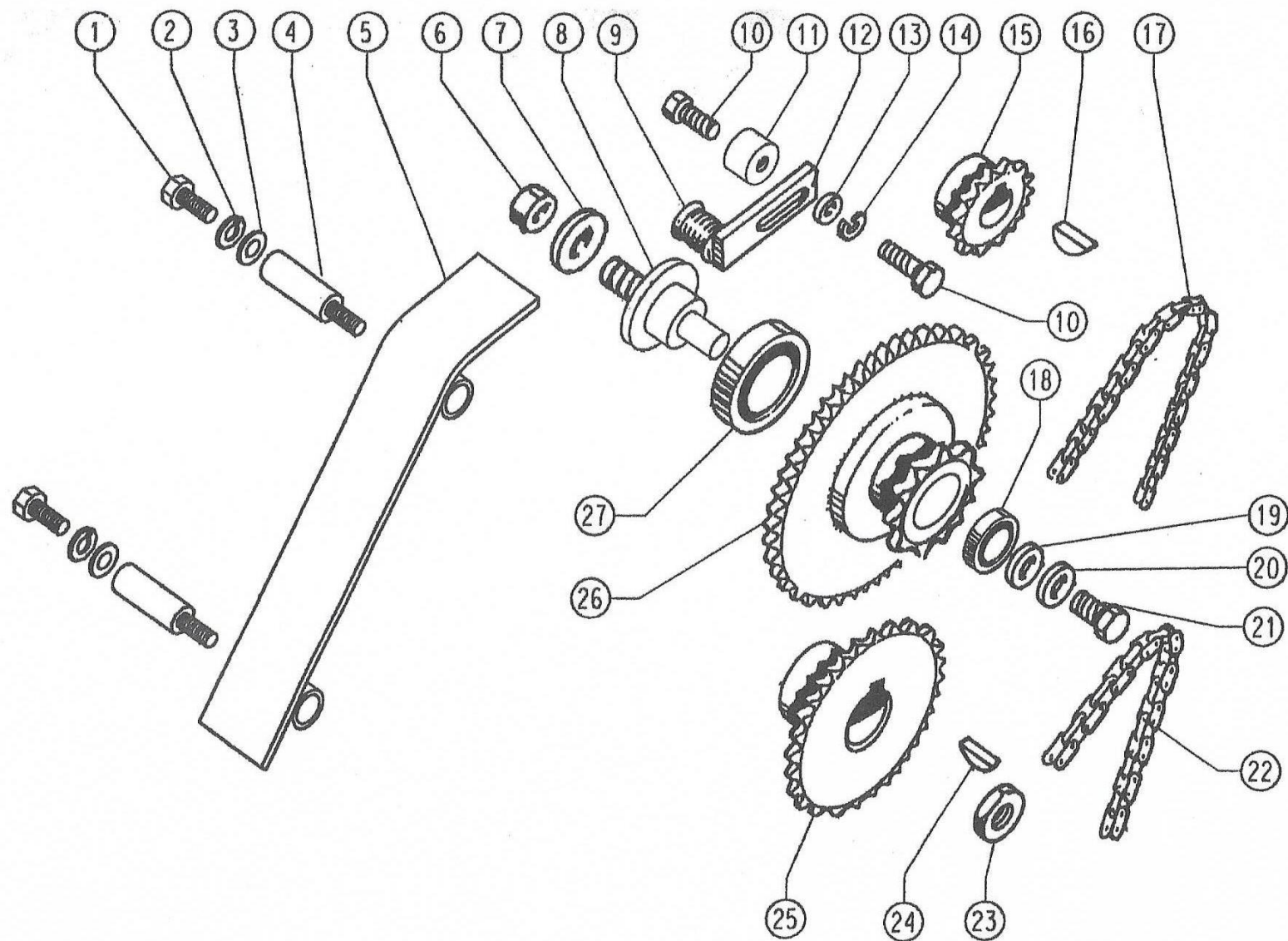
ROLLER DRIVE ASSY
