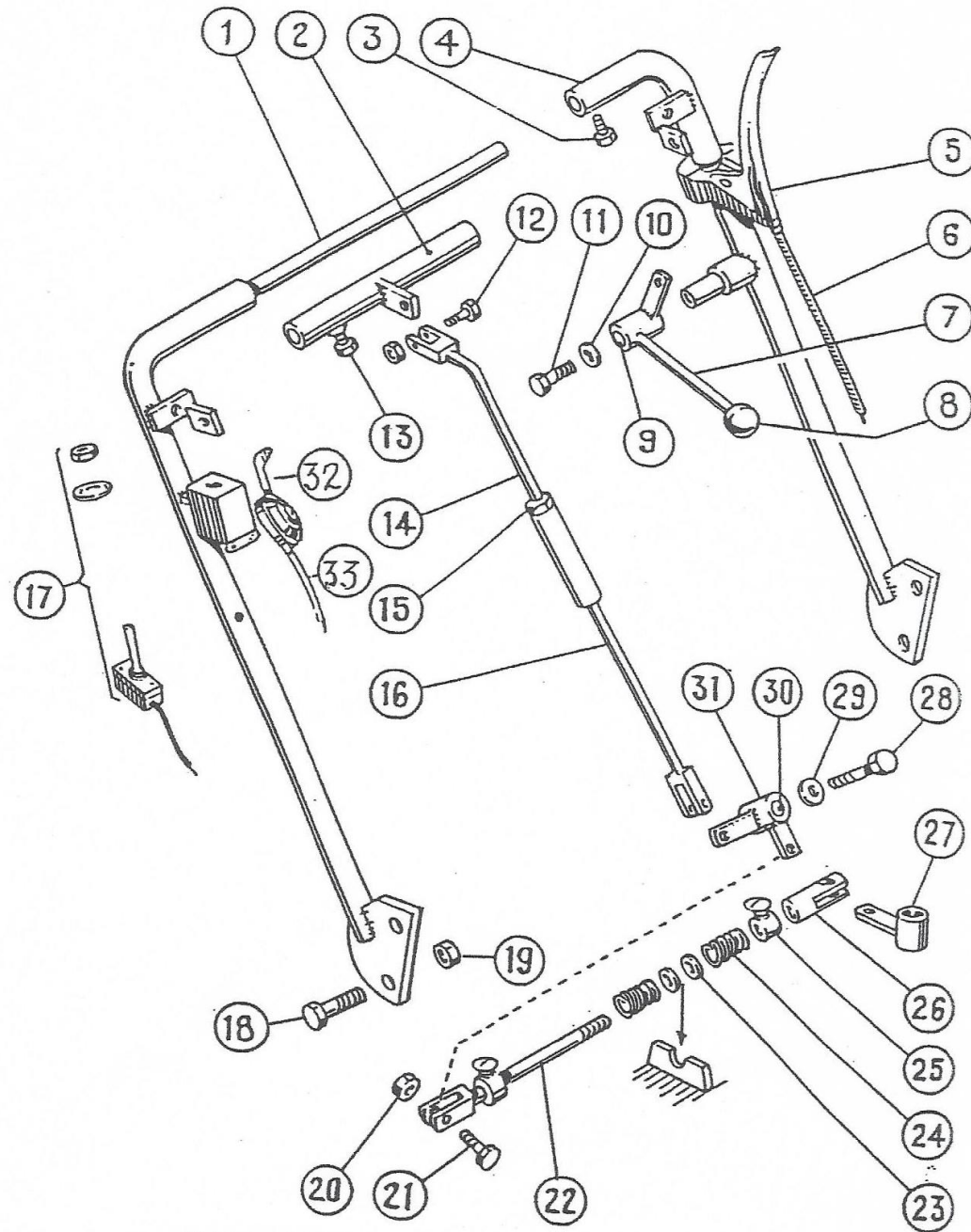
HANDLEBAR ASSY.
